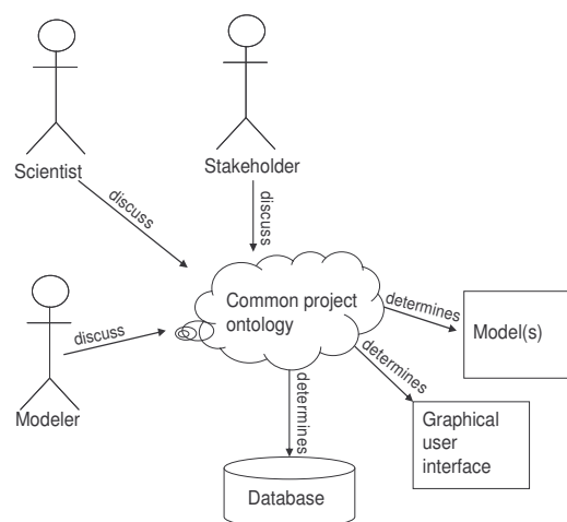
Figure 1 Role of a common project ontology in an integrated assessment modelling project
