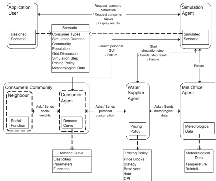
Figure 4: AORML External Agent Diagram
