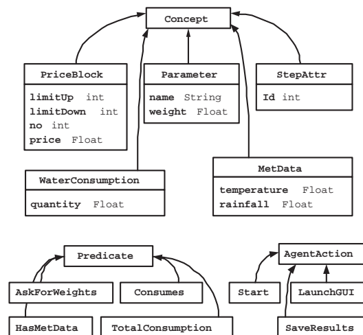
Figure 5: Water Demand-Supply Ontology: Concepts, Predicates and AgentActions
